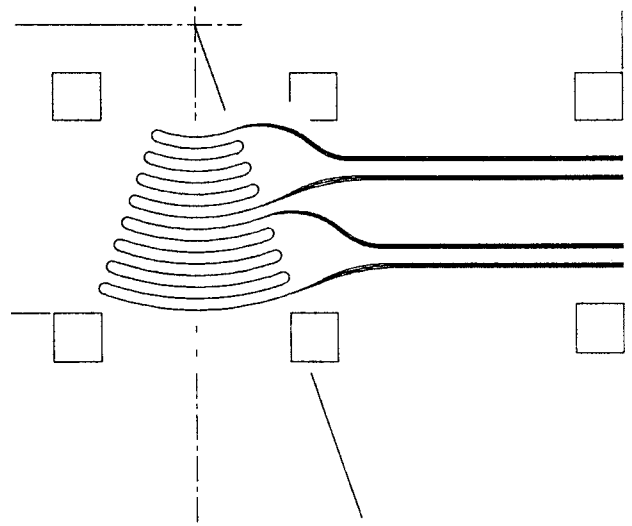
FIG. 6 Collinear-Focused EMAT Coils for Surface Wave Transduction
