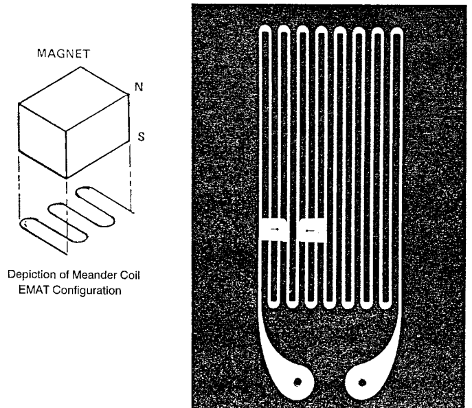
FIG. 4 Typical EMAT Meander Coil for Rayleigh Wave Generation
